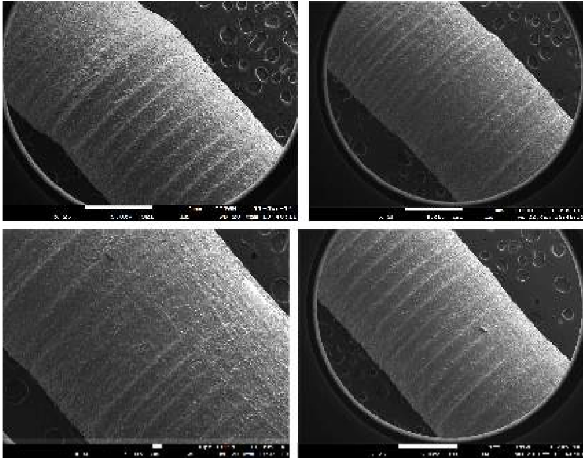
Figure 24: Bead hole impressions analysis using SEM; bead holes formed by diamond tipped steel drill from a modern bead manufactured at Khambhat
