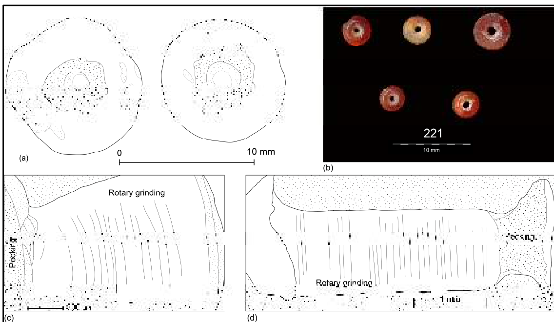
Figure 5: (a) Carnelian bead, Type 3 Pecking technology from pre-Indus Mehrgarh; (b) carnelian bead from Harappan period, Karanpura, Rajasthan showing pecking technique; (c) carnelian bead, Chalcolithic, pecking from left and rotary grinding from right; and (d) carnelian bead, pre-Indus, rotary grinding from left and pecking from right (after Barthelemy and Rodiere 2005)
