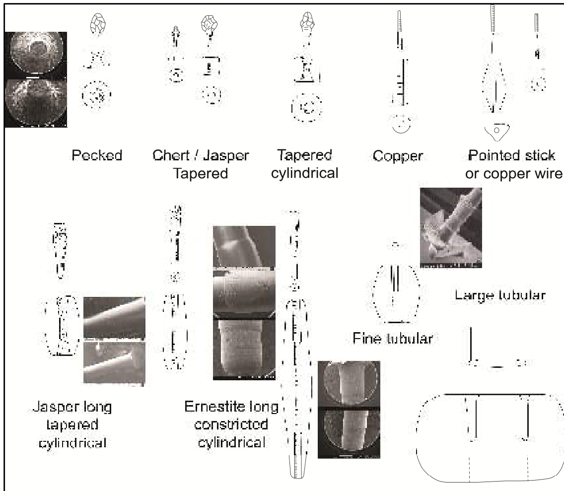
Figure 22: Drilling Patterns from Different Materials (after Kenoyer: 2003)
