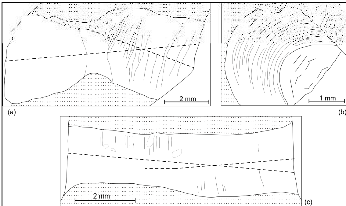
Figure 3: Type 1 drilling technology from Neolithic Mehrgarh; (a) calcite bead, dotted line showing different drilling axes meeting at the junction at centre; (b) calcite bead, showing very strong obliquity and (c) steatite bead, dotted line showing different drilling axes (after Barthelemy and Rodiere 2005)
