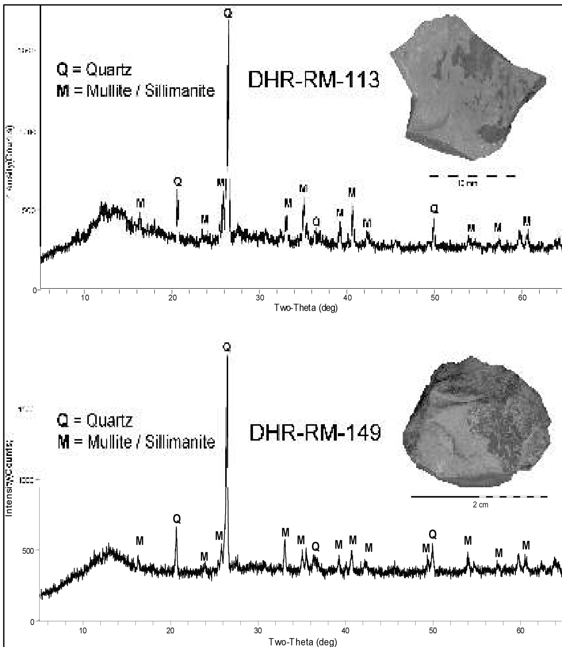
Figure 18: XRD Analysis of Ernestite, Dholavira
