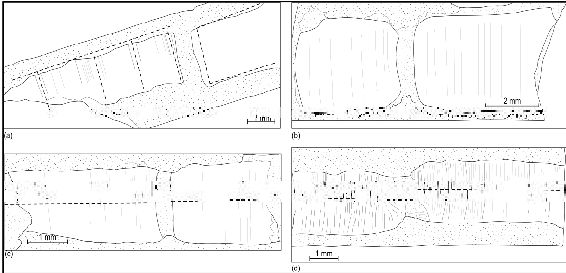
Figure 4: Type 2 drilling technology from Chalcolithic and pre-Indus Mehrgarh; (a) steatite bead, perforation identified in at least four stages; (b) carnelian bead, Chalcolithic (c) carnelian bead, pre-Indus and (d) serpentine bead, pre-Indus (after Barthelemy and Rodiere 2005)
