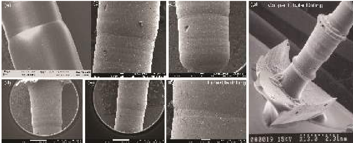
Figure 23: Bead hole impressions analysis using SEM; (a) – (f) bead holes formed by ernestite drills, (a) from Dholavira, (b) – (f) from Karanpura; (g) bead holed formed by copper tubular drill (courtesy J.M. Kenoyer)
